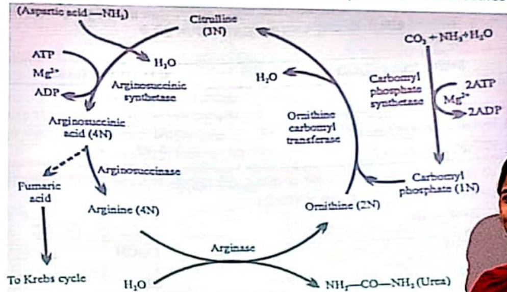
Fig. 12-1. Ornithine cycle.
